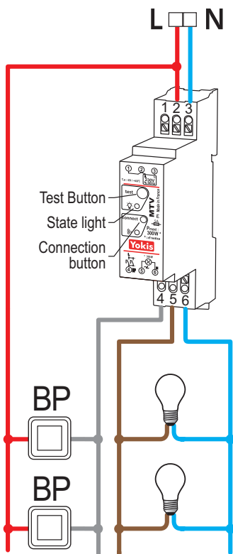
Standard connection scheme
